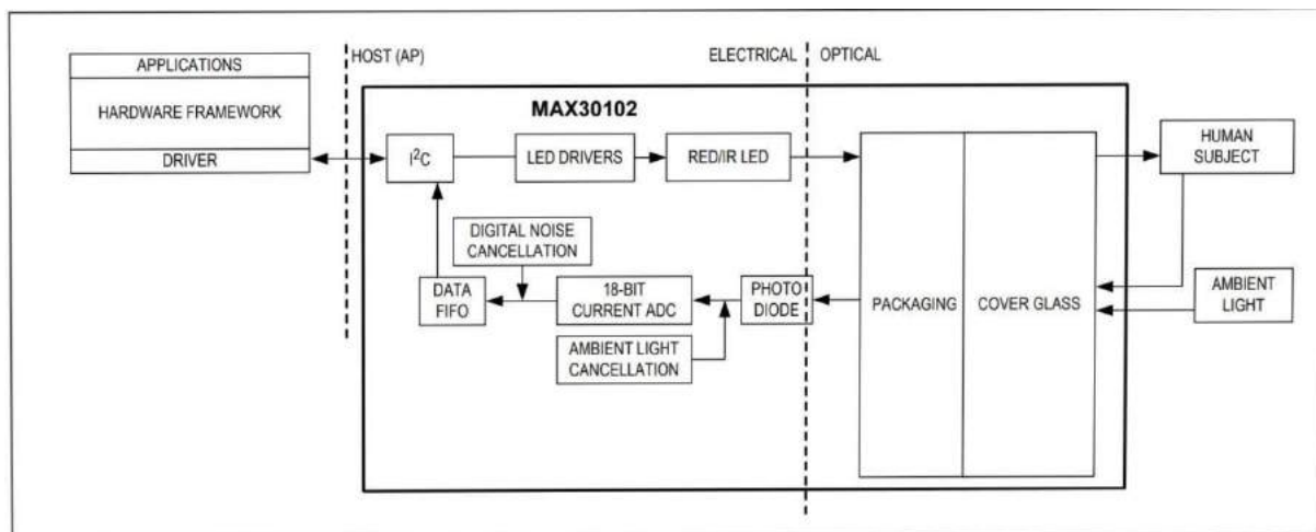
FIGURE 5 MAX30102 SENSOR
