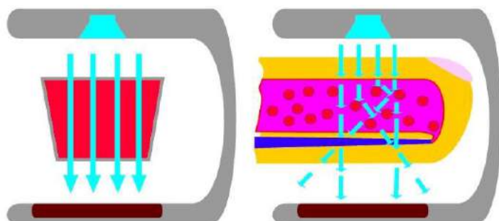
Figure 1. oxygenated haemoglobin in our blood absorbs more infrared light and red light easily passes through blood and vice-versa for deoxygenated haemoglobin
